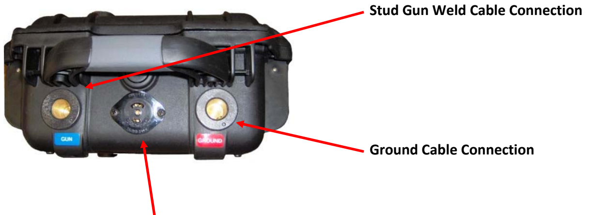
Stud Gun Control Cable Connection
